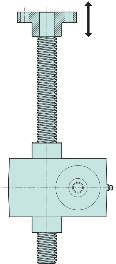
Model A – travelling screw
