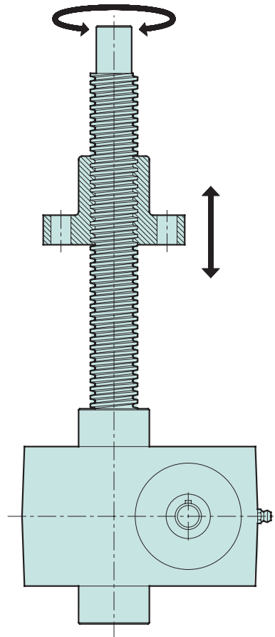
Model B – travelling nut
